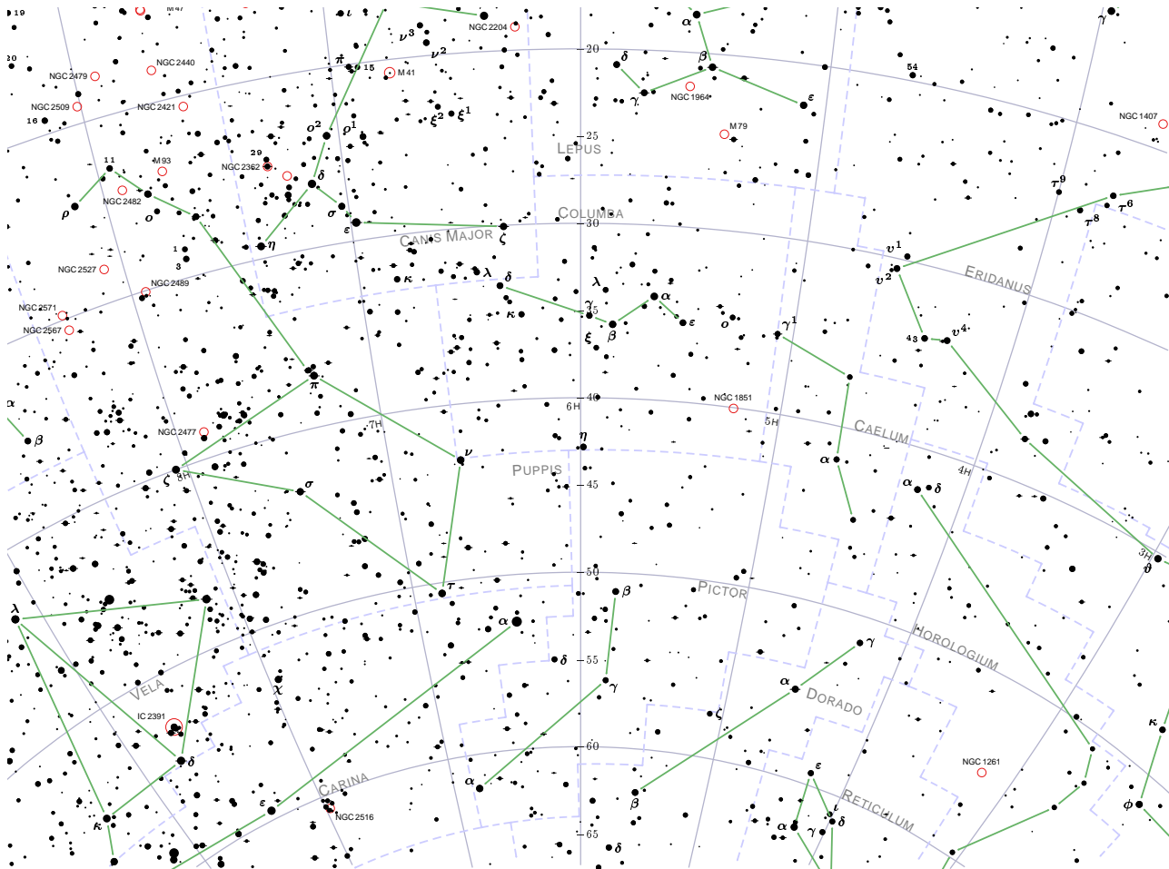
Chart 15: RA 4 h to 8 h , Declination -20° to -65°
