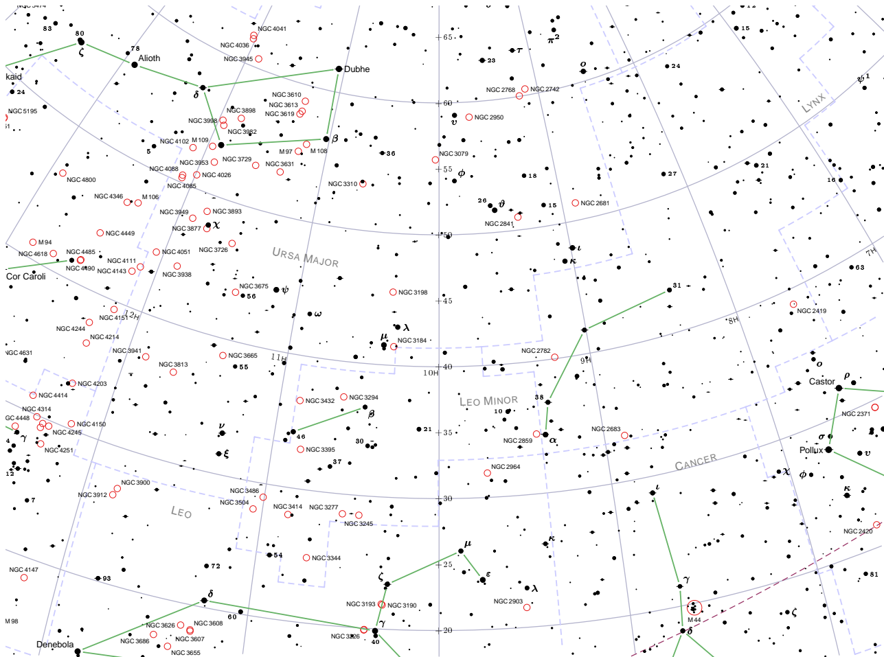
Chart 4: RA 8 h to 12 h , Declination +65° to +20°
