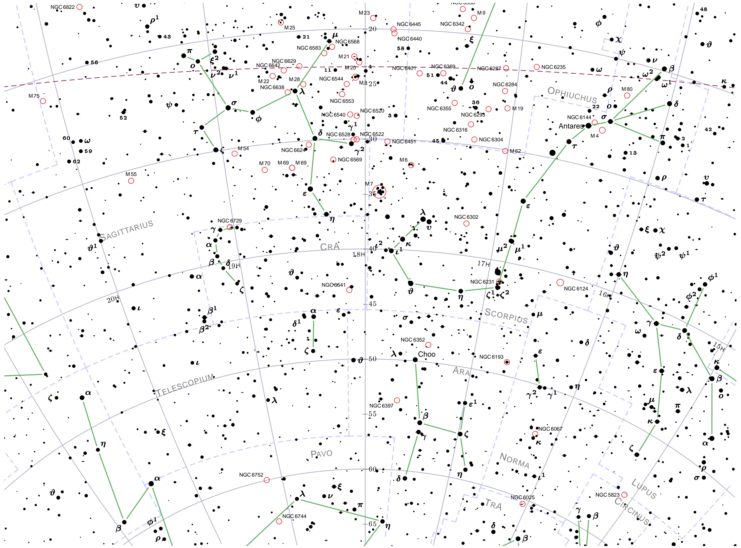
Chart 18: RA 16 h to 20 h , Declination -20° to -65°
